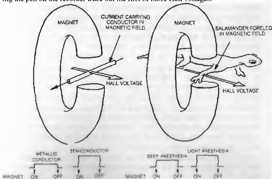
THE HALL EFFECT
